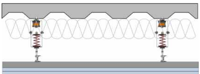
Springs Under Corrugated Deck Assembly
