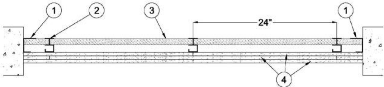
HORIZONTAL SECTION
