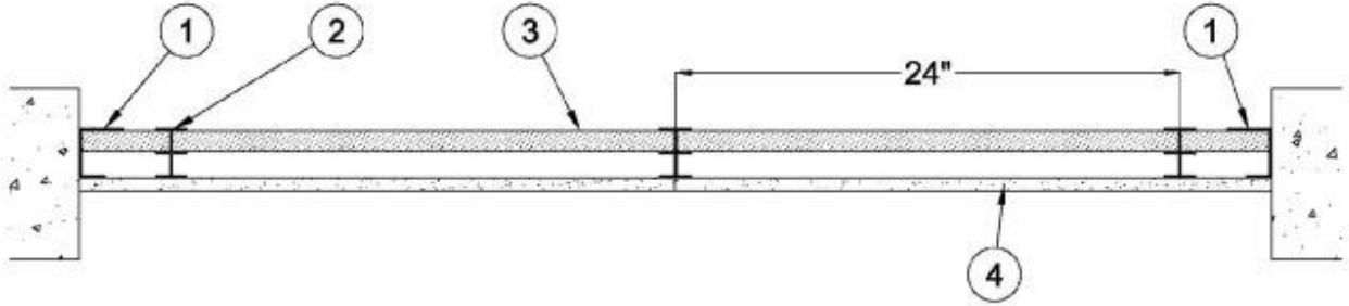
HORIZONTAL SECTION
