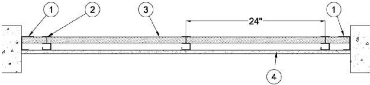
HORIZONTAL SECTION
