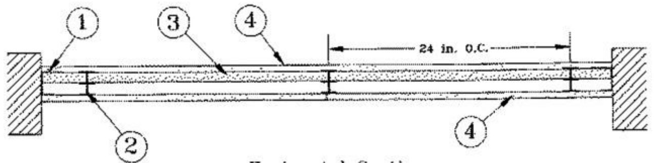
Horizontal Section System C - 2 Hr.
