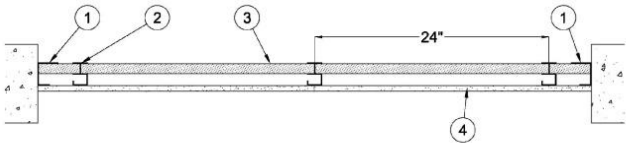
HORIZONTAL SECTION
