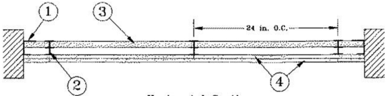
Horizontal Section System B - 2 Hr.
