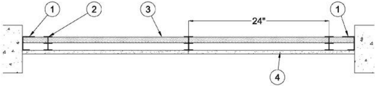
HORIZONTAL SECTION
