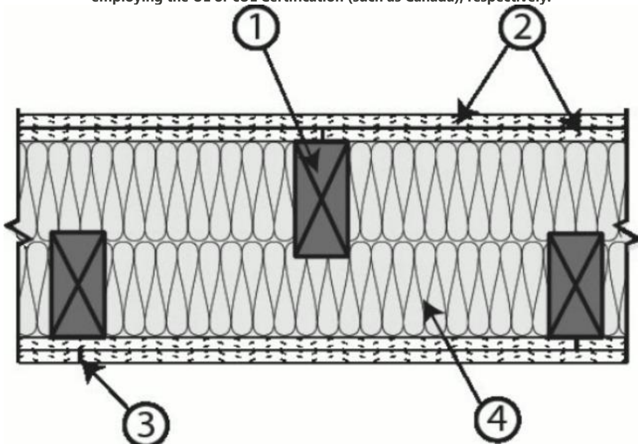
HORIZONTAL SECTION
