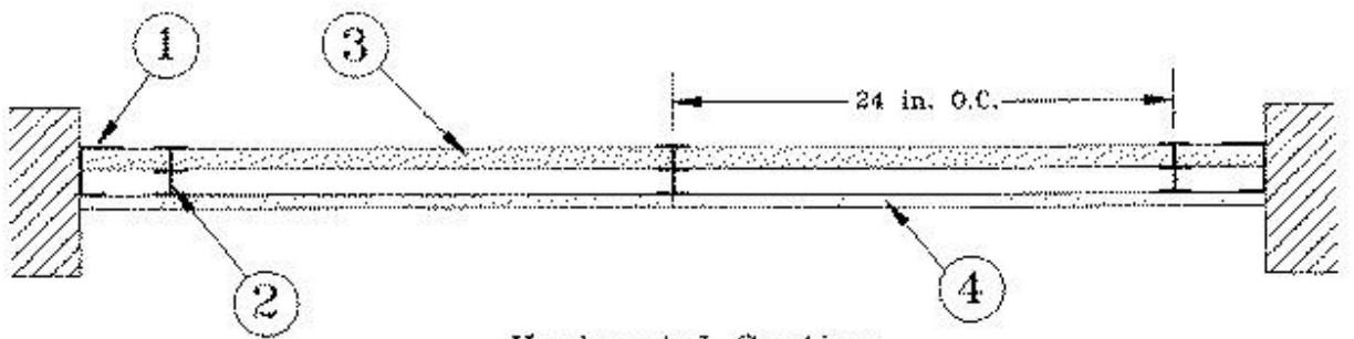
Horizontal Section
