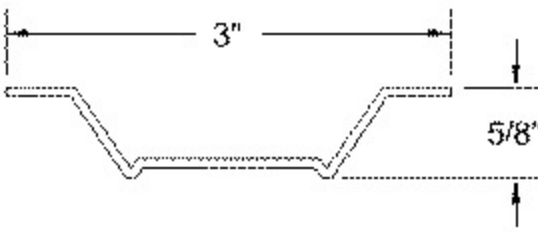
Furring Channel Detail
