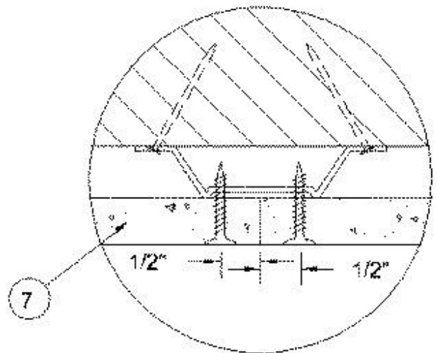
End Joint Detail
