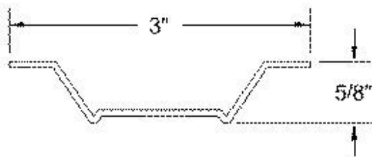
Furring Channel Detail
