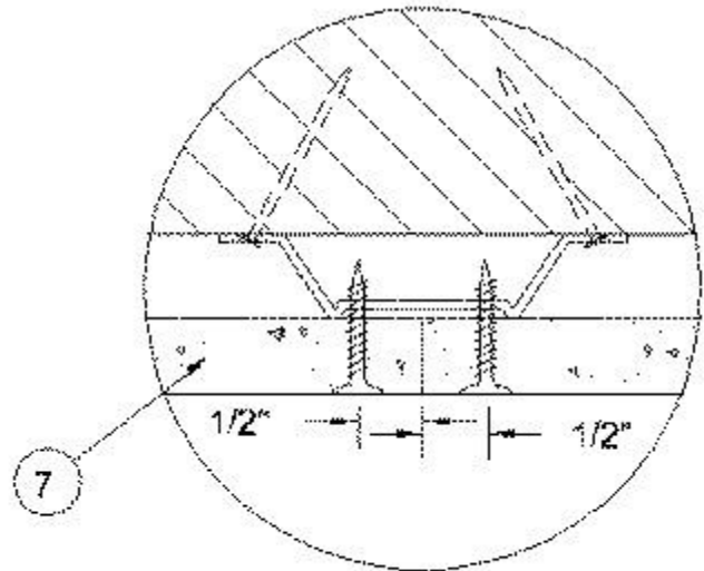
End Joint Detail
