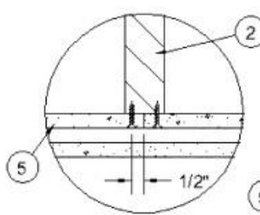
First Layer End Joint Detail
