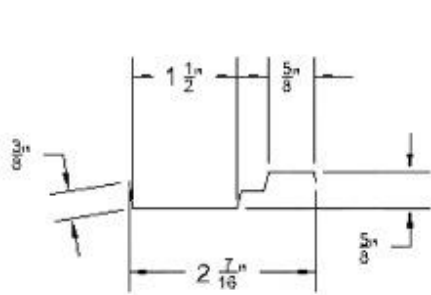
Resilient Channel Detail
