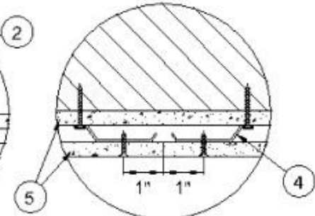
Second Layer End Joint Detail
