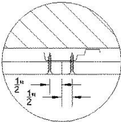
End Joint
