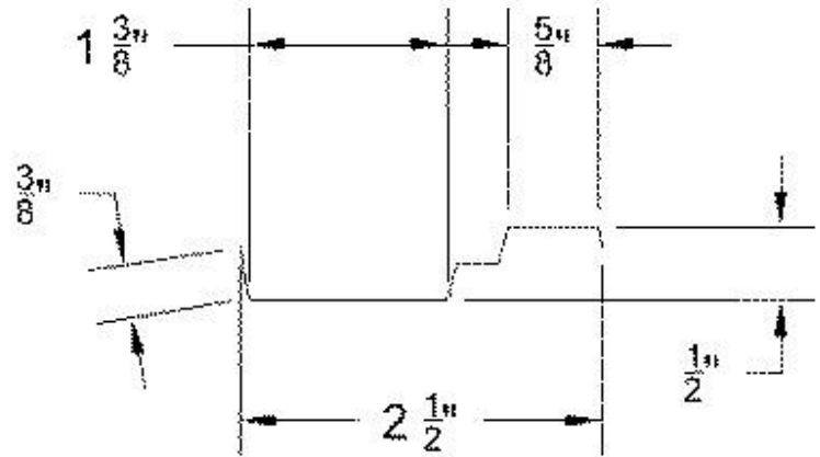
Resilient Channel Detail
