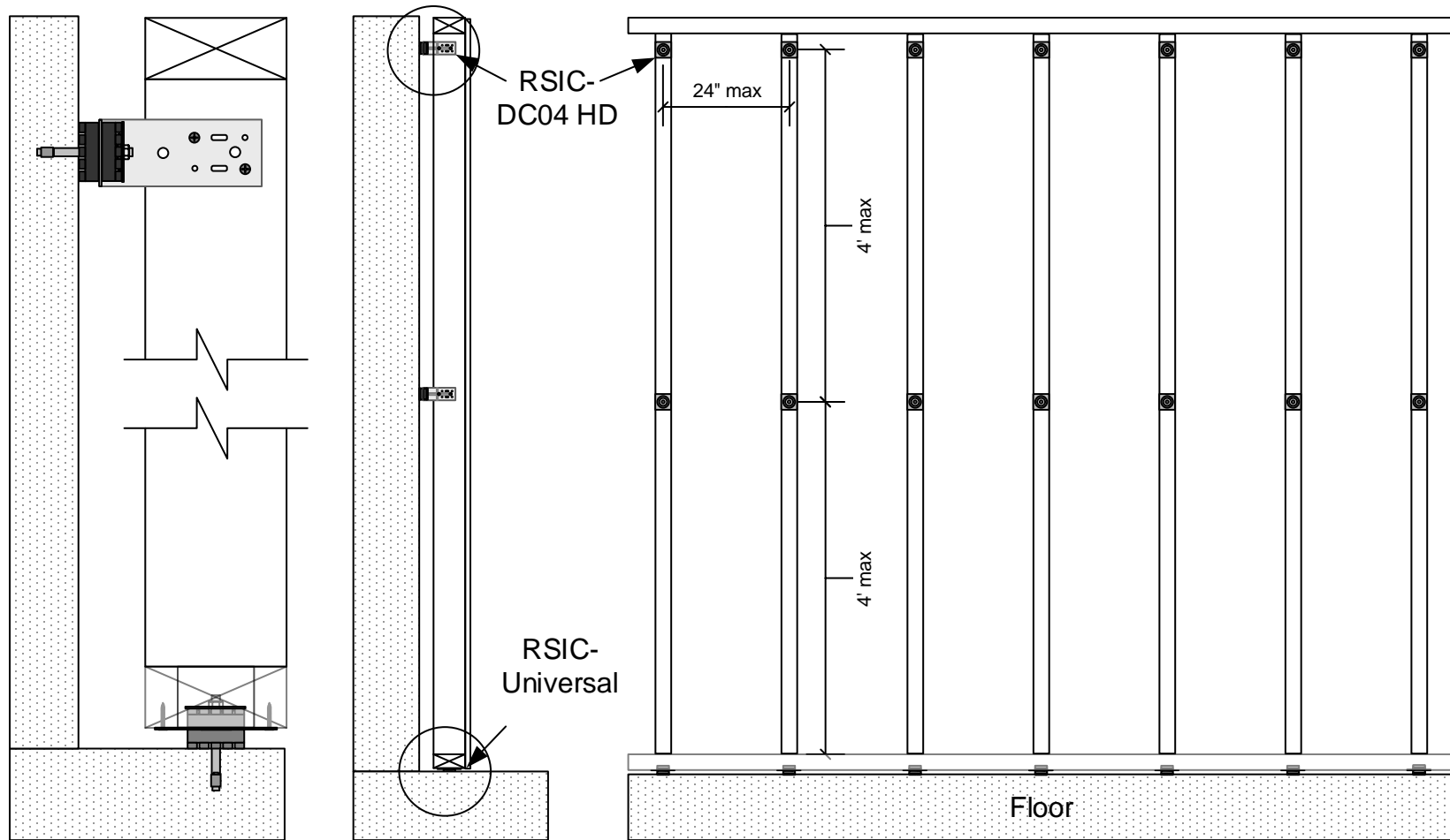
RSIC-DC04 HD/DD Mounted to the top plate. Max spacing 24" x 48" oc.
